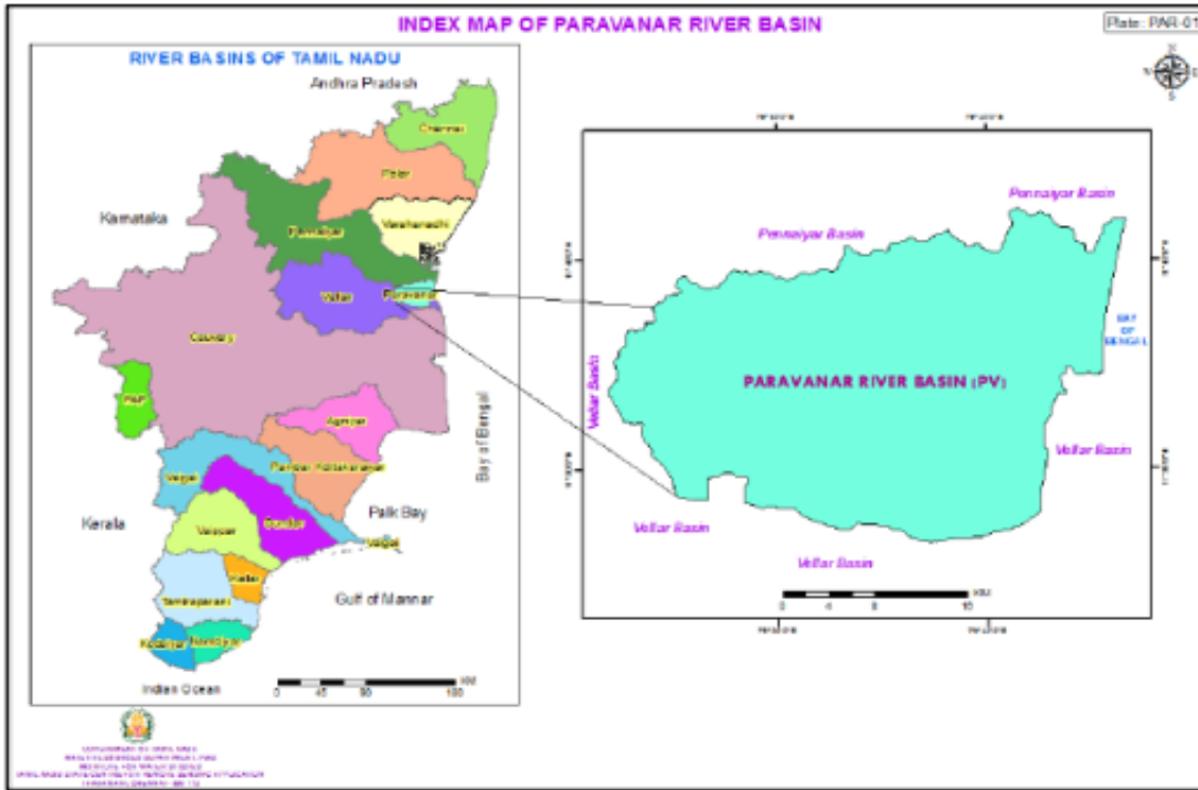
Fig. 1 Index map of Paravanar River Basin
